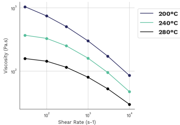
Viscosity-shear rate Rilsan® BECNO TL
