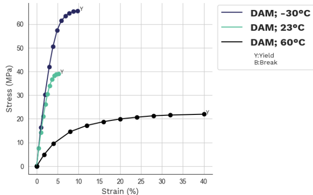
Stress-strain Rilsan® BECNO TL
