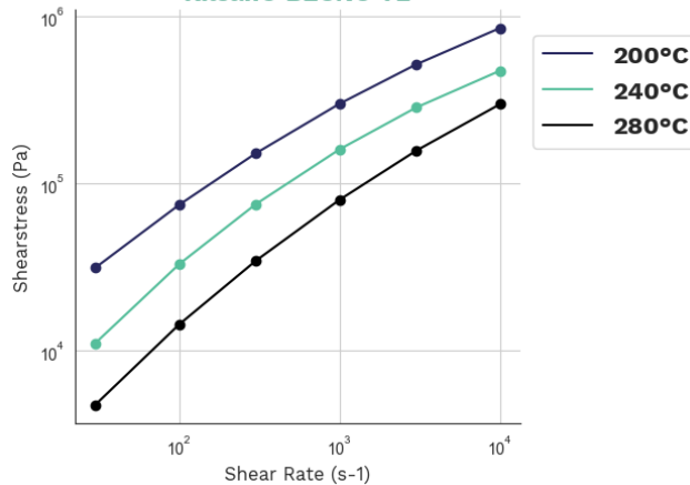
Shearstress-shear rate Rilsan® BECNO TL
